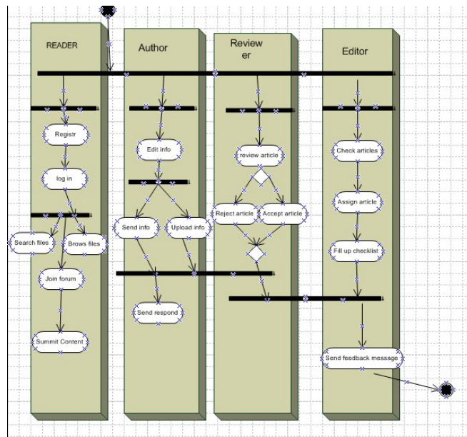
FIGURE 4. ACTIVITY DIAGRAM
